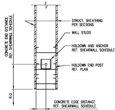
2 53.01 TYP HOLDOWN DETAIL 1 1/2" = 1'-0"
