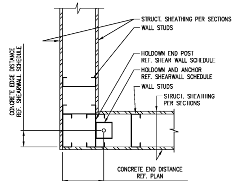
3 53.01 TYP HOLDOWN DETAIL 1 1/2" = 1'-0"
