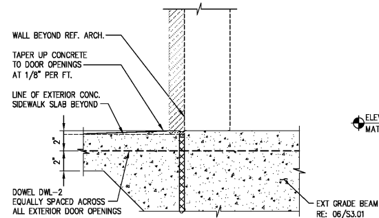
5 53.01 TYP DOOR OPENING DETAIL 1 1/2" = 1'-0"
