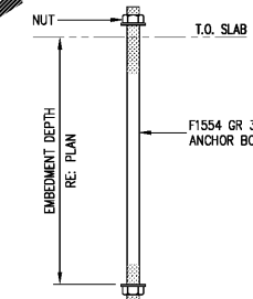
7 53.01 TYPICAL HOLDOWN ANCHOR BOLT DETAIL N.T.S.
