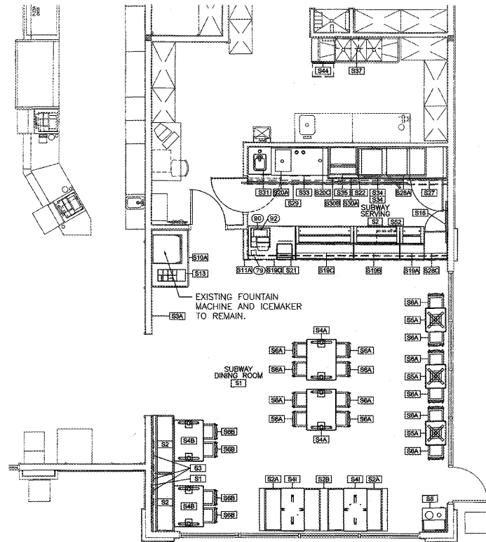
1 EQUIPMENT PLAN A3 3/16" = 1'-0"
