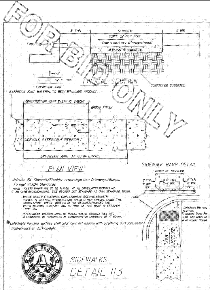
1 COBB COUNTY STANDARD SIDEWALK DETAIL
