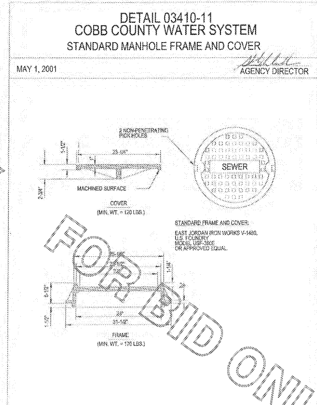
6 COBB COUNTY STANDARD MANHOLE DETAIL
