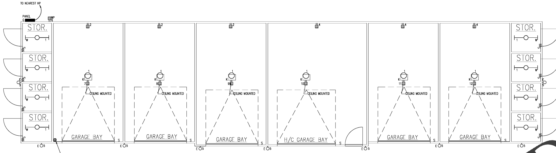
1 E-12 6 CAR HC GARAGE ELECTRICAL PLAN SCALE: 1/4" = 1'-0"
