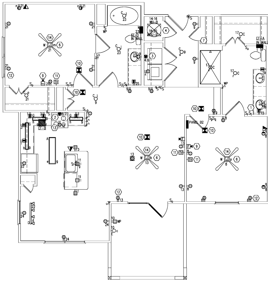
1 UNIT B2 ELECTRICAL PLAN E-4 SCALE: 1/4" = 1'-0"
