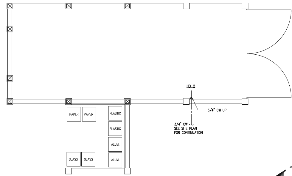
2 COMPACTOR FLOOR PLAN P-4 1/4" = 1'-0"
