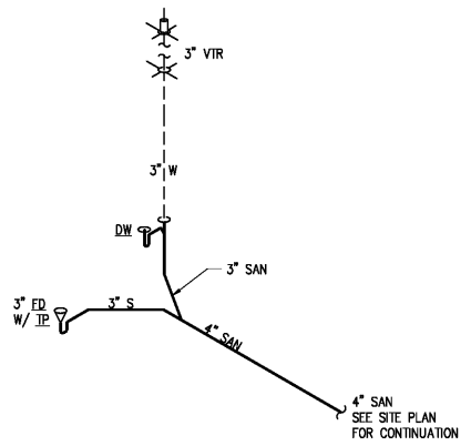
3 DOG WASH SANITARY PLAN P-4 NOT TO SCALE
