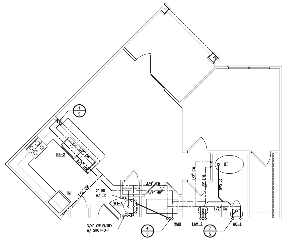
UNIT A3 FLOOR PLAN P-1 1/4" = 1'-0"
