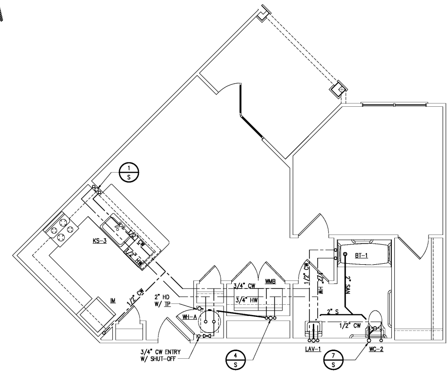
UNIT A3 HC FLOOR PLAN P-1 1/4" = 1'-0"
