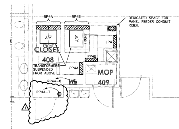
5 ENLARGED 4TH FLOOR ELECTRICAL ROOM 1/4" = 1'-0"
