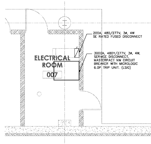
1 ENLARGED GROUND FLOOR ELECTRICAL ROOM 1/4" = 1'-0"
