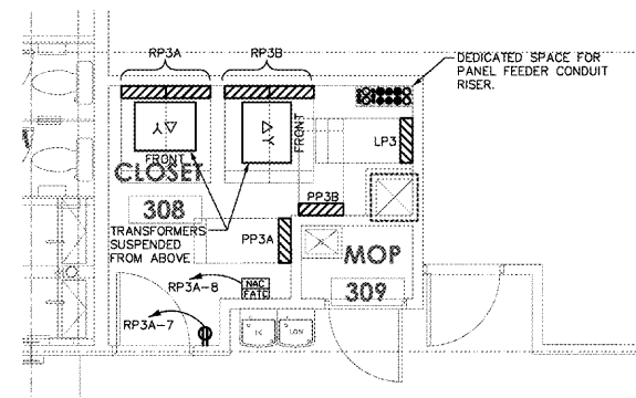
3 ENLARGED 3RD FLOOR ELECTRICAL ROOM 1/4" = 1'-0"
