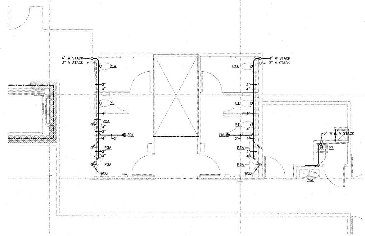
③ THIRD AND FOURTH FLOOR RESTROOMS - GRAVITY PIPING 1/4" = 1'-0"
