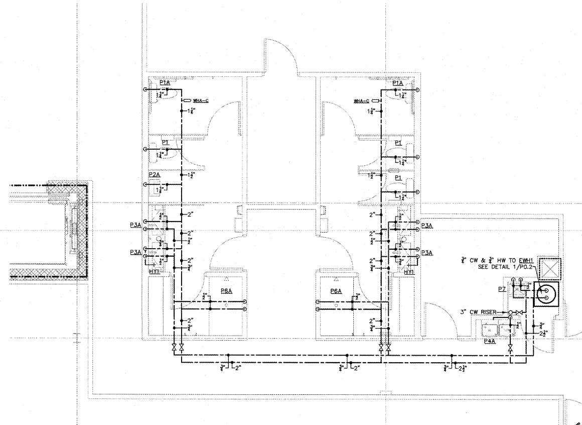
② SECOND FLOOR RESTROOMS - PRESSURE PIPING 1/4" = 1'-0"
