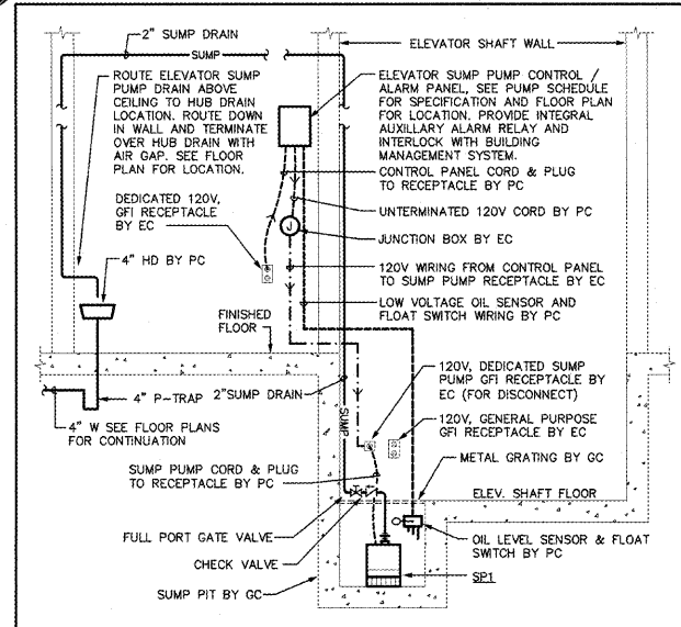
2 ELEVATOR SUMP PUMP SPI NOT TO SCALE
