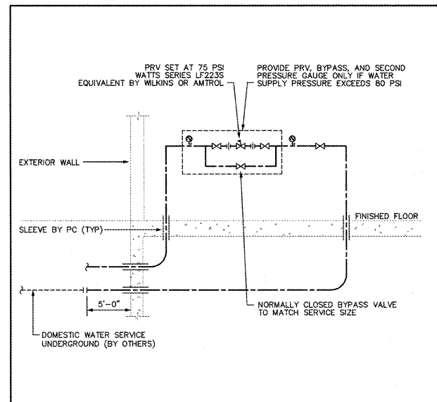
3 WATER SERVICE ENTRY FOR OFFICE BUILDING NOT TO SCALE
