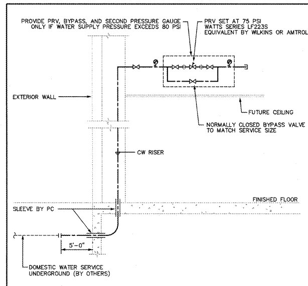
6 WATER SERVICE ENTRY AT FUTURE RESTAURANT NOT TO SCALE
