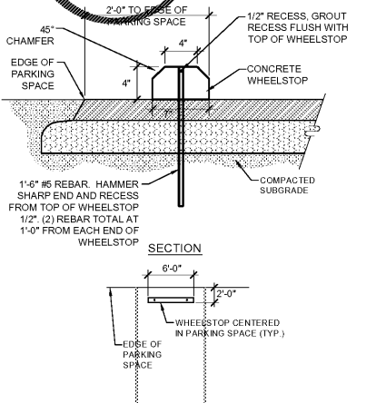
ASPHALT WHEELSTOP DETAIL NTS
