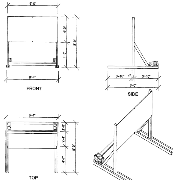
1 COMING SOON TEMPORARY CONSTRUCTION SIGN SQ1.2 SCALE: 1/4" = 1'-0"
