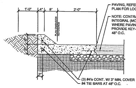
3 CONCRETE CURB SECTION C2.2 SCALE: 2/4" = 1'-0"
