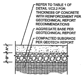
1 CONCRETE PAVING SECTION C2.2 SCALE: NOT TO SCALE
