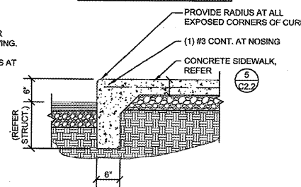
4 CONCRETE SIDEWALK CURB SECTION C2.2 SCALE: 3/4" = 1'-0"
