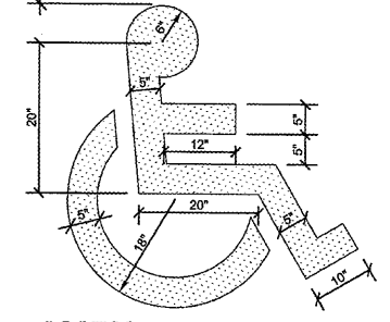
6 ACCESSIBLE PARKING PAVEMENT STRIPPING DETAIL C2.2 SCALE: 3/4" = 1'-0"
