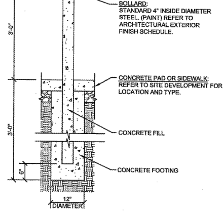
7 STEEL BOLLARD SECTION C2.2 SCALE: 3/4" = 1'-0"
