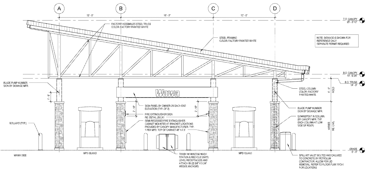
27 CANOPY ELEVATION 14' x 14'
