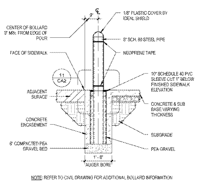
5 BOLLARD DETAIL 12" x 12"
