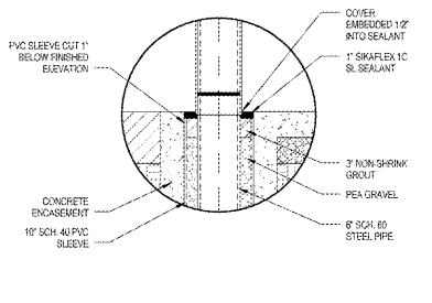
11 ENLARGED BOLLARD DETAIL 12" x 12"
