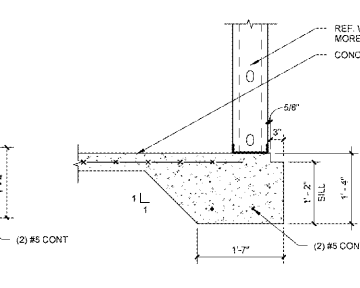
(15) THICKENED EDGE - WITH CURB
