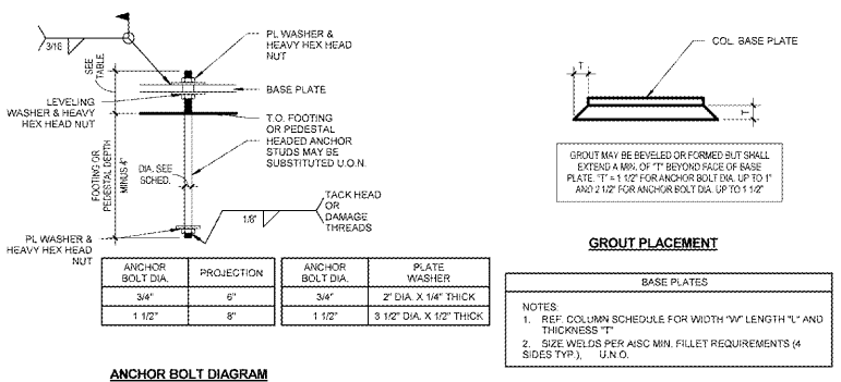
ANCHOR BOLT DIAGRAM
