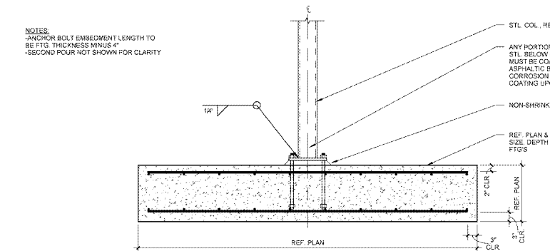
(8) FOUNDATION DETAIL
