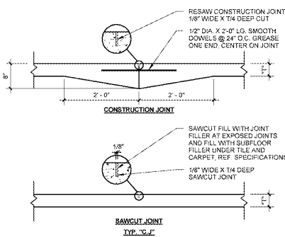
(3) GENERAL CONSTRUCTION JOINT INFORMATION
