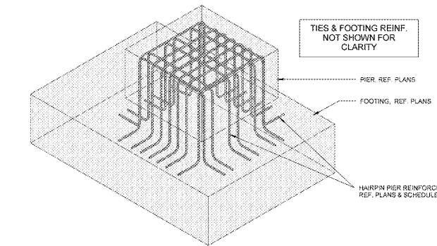
(19) PIER #2 ISO
