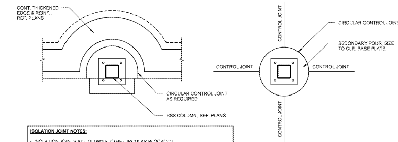
(2) GENERAL ISOLATION JOINT INFORMATION
