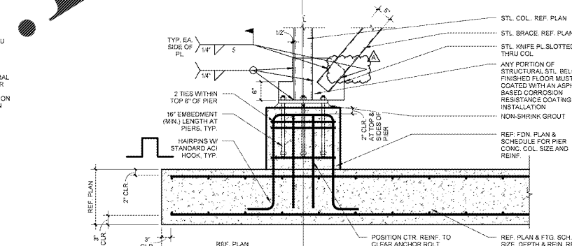
(10) FOUNDATION DETAIL
