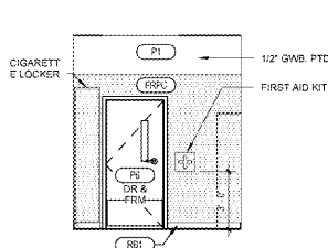
17 ASSOCIATE'S ROOM ELEV. A8.2 1/4" x 1'-0"
