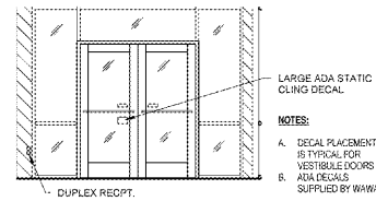
5 ADA DECAL DTL @ VESTIBULE DOOR A8.2 1/4" x 1'-0"
