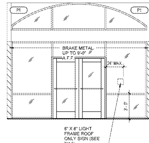
3 FRONT VESTIBULE ELEVATION A8.2 1/4" x 1'-0"
