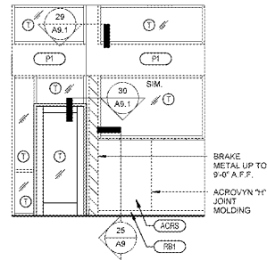
4 FRONT VESTIBULE ELEVATION A8.2 1/4" x 1'-0"
