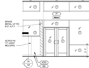
2 FRONT VESTIBULE ELEVATION A8.2 1/4" x 1'-0"
