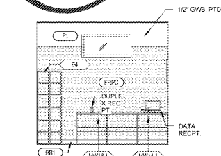
18 ASSOCIATE'S ROOM ELEV. A8.2 1/4" x 1'-0"
