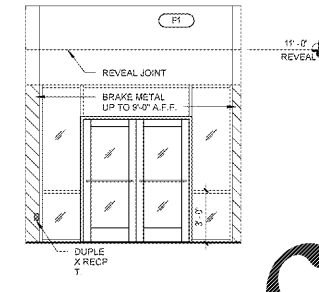
1 FRONT VESTIBULE ELEVATION A8.2 1/4" x 1'-0"
