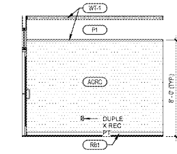
9 REAR VESTIBULE ELEVATION A8.2 1/4" x 1'-0"
