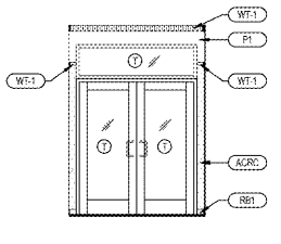
8 REAR VESTIBULE ELEVATION A8.2 1/4" x 1'-0"
