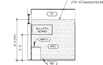
16 ASSOCIATE'S ROOM ELEV. A8.2 1/4" x 1'-0"
