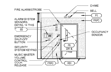
11 OFFICE ELEVATION A8.2 1/4" x 1'-0"
