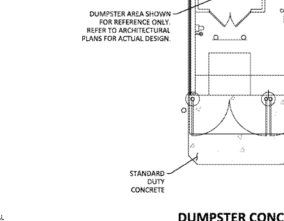
DUMPSTER CONCRETE APRON NTS
