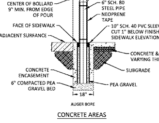
CONCRETE AREAS NTS
