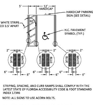
HANDICAP STRIPING DETAIL NTS
