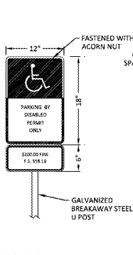
HANDICAP PARKING SIGN NTS
