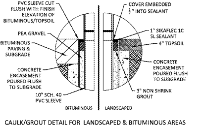
CAULK/GROUT DETAIL FOR LANDSCAPED & BITUMINOUS AREAS NTS
