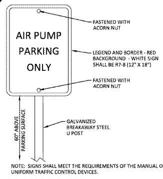
AIR PARKING SIGN NTS
