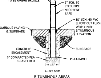
BITUMINOUS AREAS NTS
