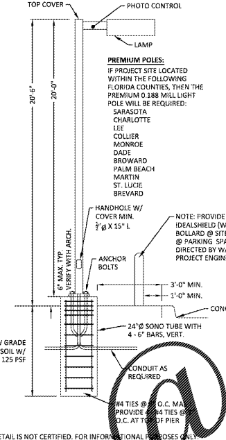
LIGHT POLE WITH STANDARD ANCHORING DETAIL NTS
