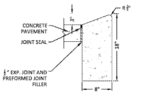
WAWA TYPE B1 CURB NTS
