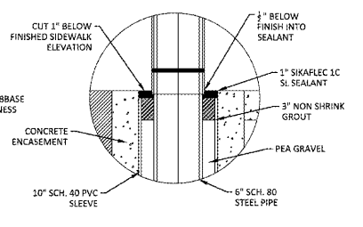
GENERAL DETAILS AND CAULK/GROUT DETAIL FOR CONCRETE AREAS NTS
