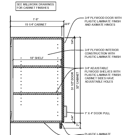
6C GUEST EXPERIENCE UPPER CABINET 1 1/2" = 1'-0"
