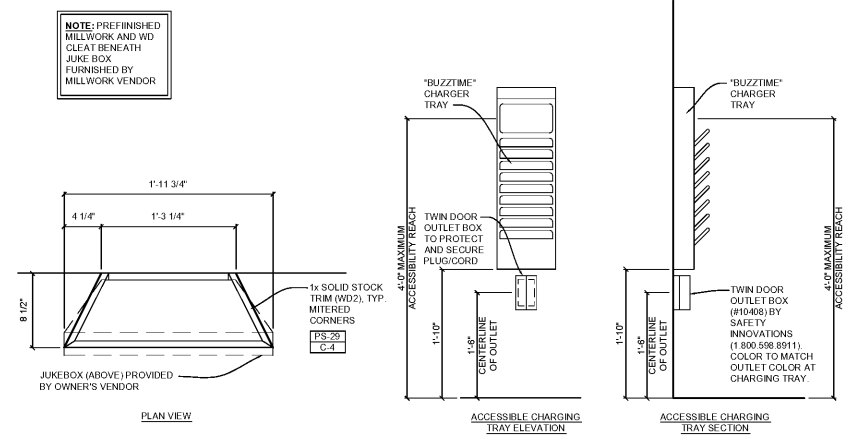
4B CHARGER TRAY & BOX MOUNTING 1" = 1'-0"
