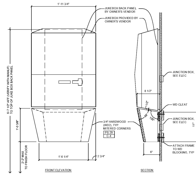
1B JUKE BOX DETAILS 1 1/2" = 1'-0"
