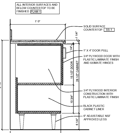
6E SERVER STATION BASE CABINET 1 1/2" = 1'-0"
