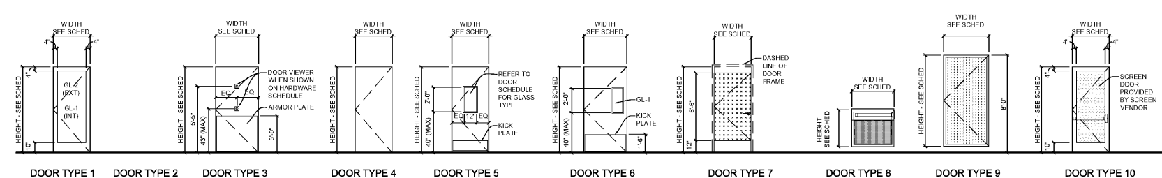
1A TYPICAL DOOR TYPES 1/4" = 1'-0"
