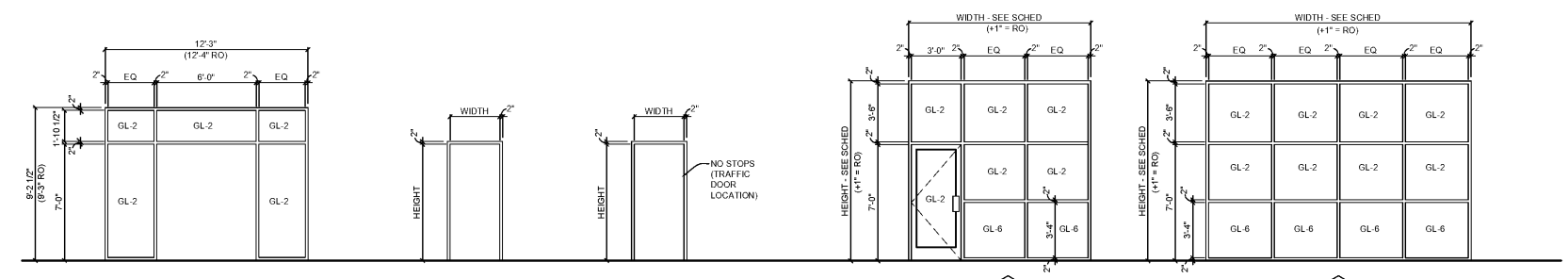
1B TYPICAL FRAME TYPES 1/4" = 1'-0" 1C TYPICAL WINDOW TYPES 1/4" = 1'-0"
