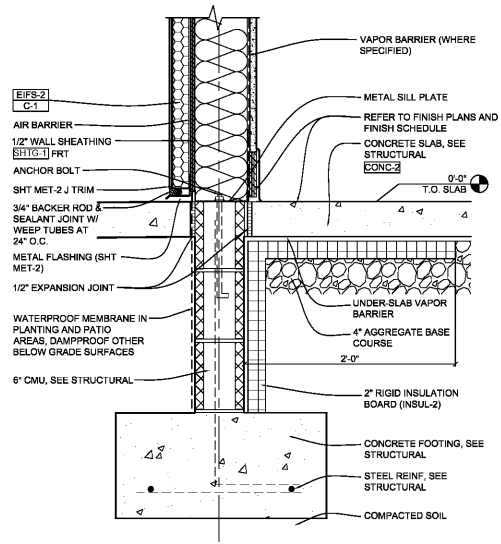
2B FOOTING DETAIL 1 1/2" x 1'-0"
