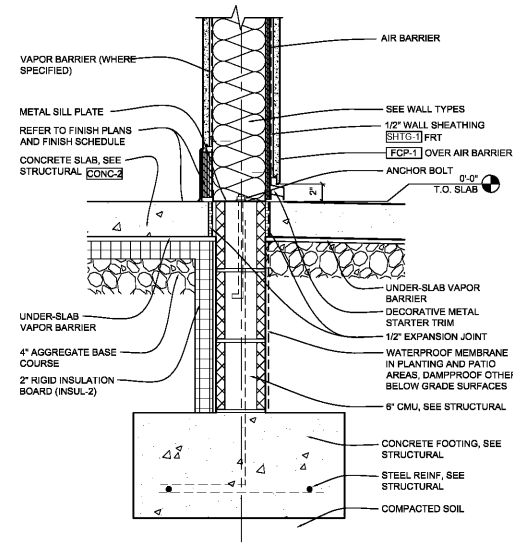
4B FOOTING DETAIL 1 1/2" x 1'-0"
