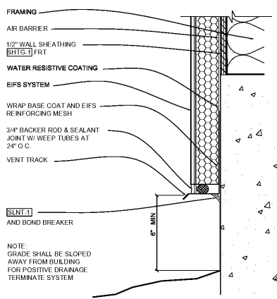
2E TYP TERMINATION AT FOUNDATION 3" x 1'-0"
