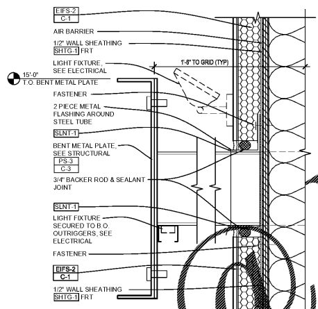
2D STEEL CHANNEL BEAM DETAIL 3" x 1'-0"
