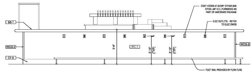
5D BAR ELEVATION 1/2" = 1'-0"
