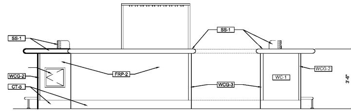
1B BAR ELEVATION 1/2" = 1'-0"
