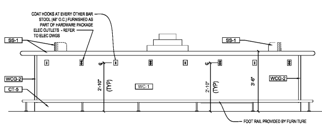
3D BAR ELEVATION 1/2" = 1'-0"
