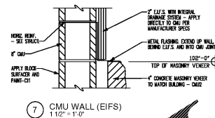
7 CMU WALL (EIFS) 1/12" = 1'-0"
