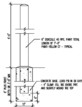
9 BOLLARD DETAIL 3/4" = 1'-0"
