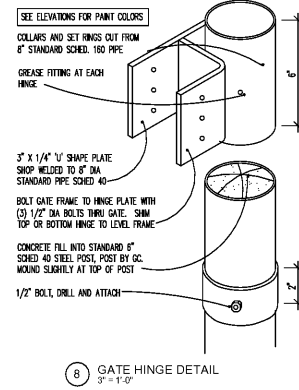
8 GATE HINGE DETAIL 3/4" = 1'-0"
