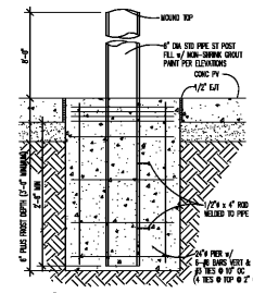
5 GATE POST 3/4" = 1'-0"
