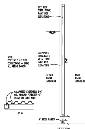
4 GATE DETAIL 3/4" = 1'-0"
