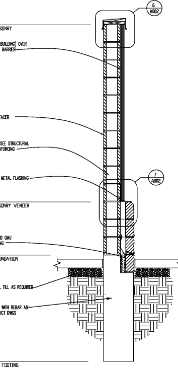
3 WALL SECTION 3/4" = 1'-0"
