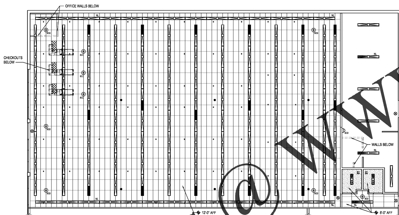
REFLECTED CEILING PLAN SCALE: 1/8" = 1'-0"
