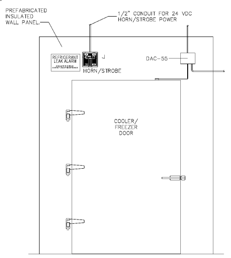
4 CONTROL SYSTEM - REFRIGERANT LEAK HORN/STROBE MOUNTING DETAIL
