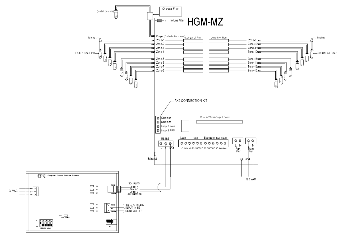
1 REFRIGERANT LEAK DETECTION UNIT - HGM MZ
