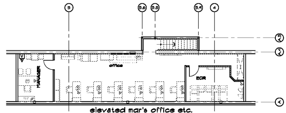
REFRIGERATION LEAK DETECTION PLAN - ELEVATED OFFICE SCALE: NOT TO SCALE
