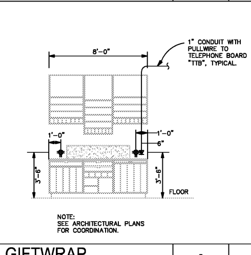
GIFTWRAP COUNTER DETAIL 3 NOT TO SCALE
