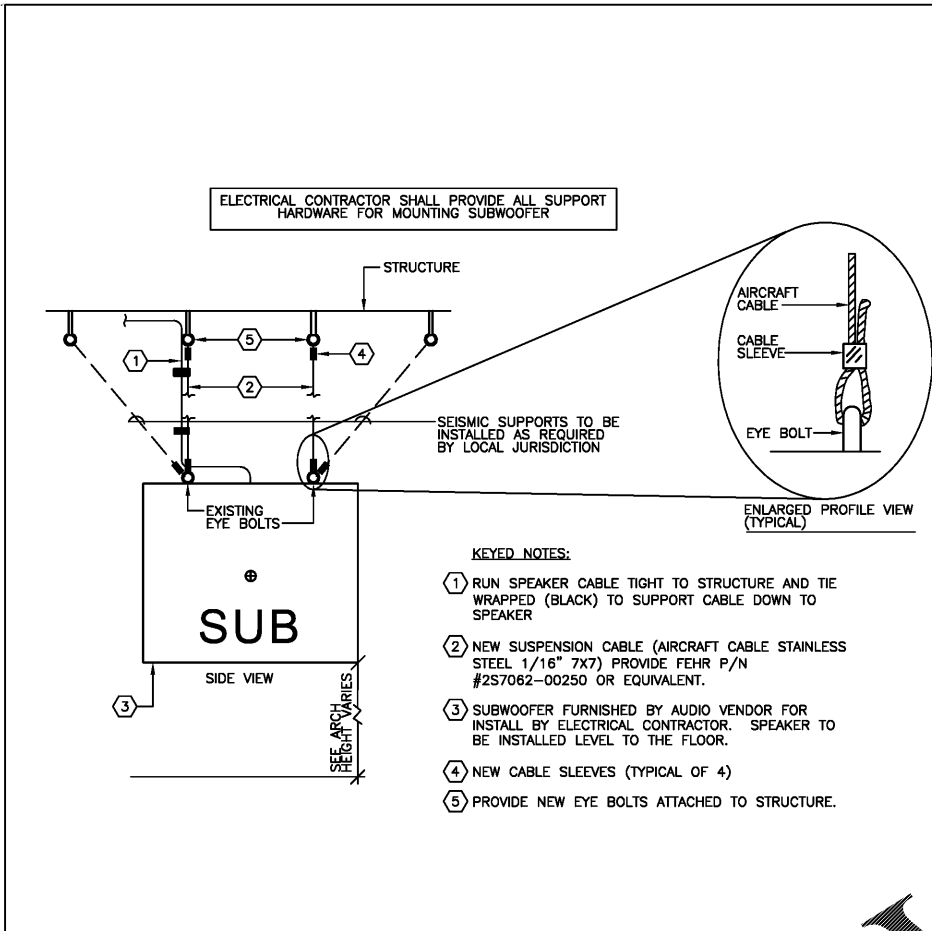
TYPICAL SUBWOOFER DETAIL 6 NOT TO SCALE
