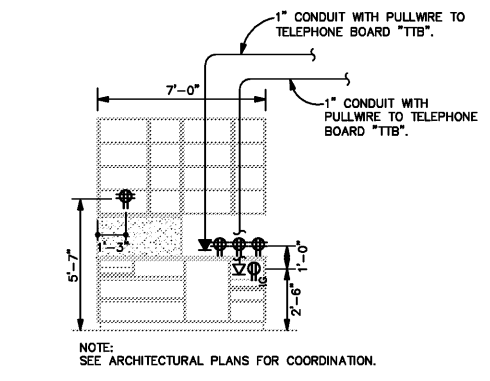
SHIPPING/RECEIVING COUNTER DETAIL 2 NOT TO SCALE
