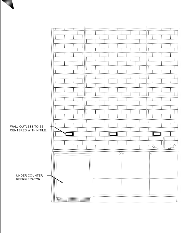
COFFEE BAR DETAIL 5 NOT TO SCALE
