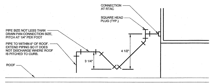
RTAC CONDENSATE DRAIN TRAP PIPING DETAIL NO SCALE
