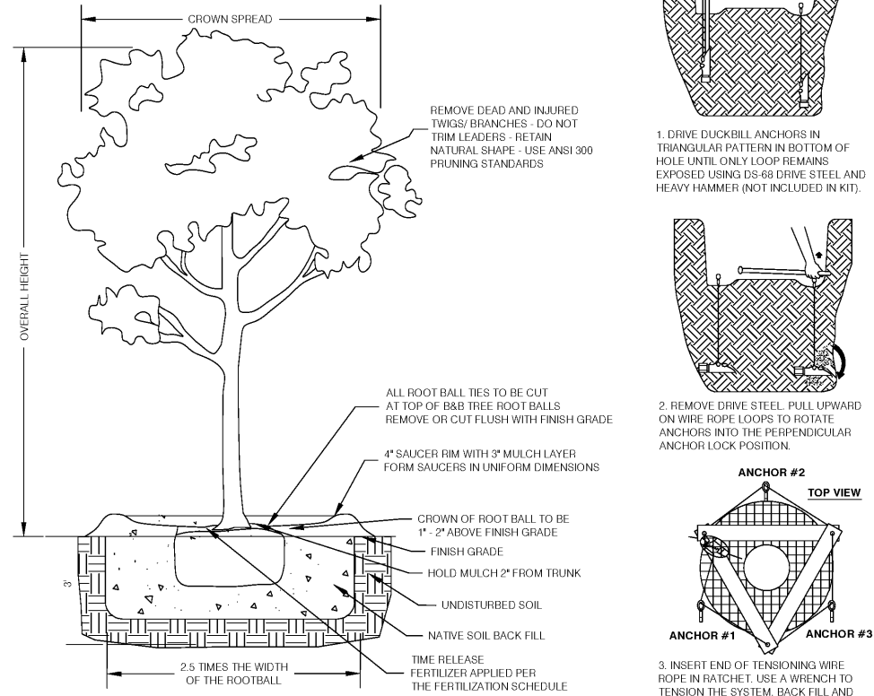
1 LARGE TREE PLANTING DETAIL (3" OR GREATER CALIPER) LS2 NOT TO SCALE
