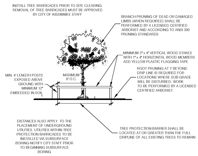
5 TREE PROTECTION DETAIL LS2 NOT TO SCALE
