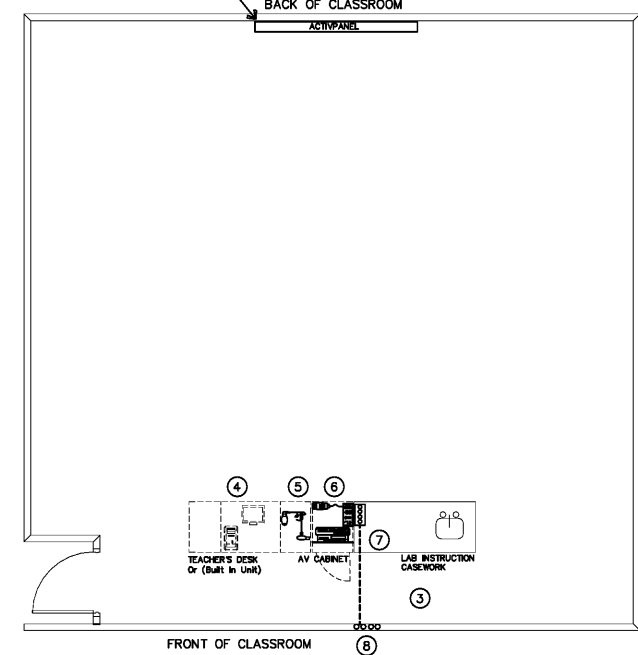
2 TYP. LAB/SCIENCE CLASSROOM A/V EQUIPMENT PLACEMENT [AVC-2] SCALE: NONE
