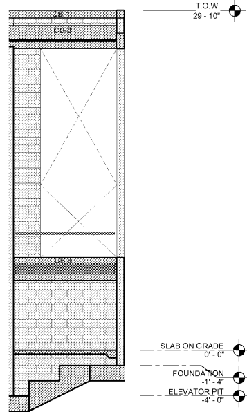
E17 ELEVATION 17 S5.3 SCALE: 3/16" = 1'-0"
