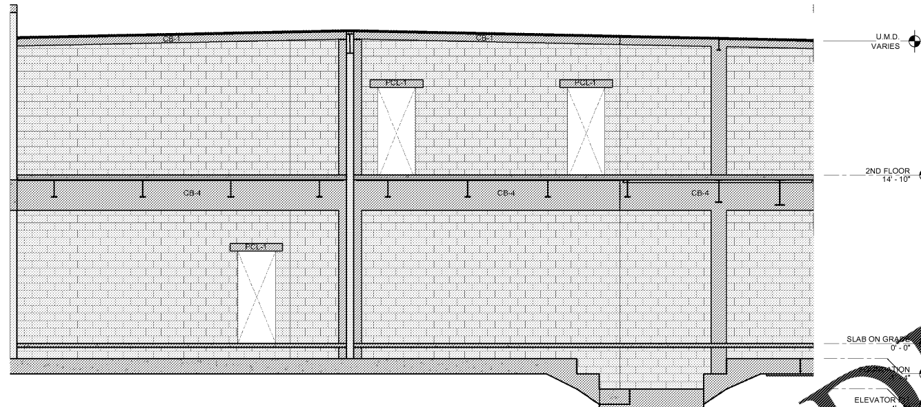
E18 ELEVATION 18 S5.3 SCALE: 3/16" = 1'-0"
