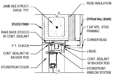
22 JAMB DETAIL SCALE: 1/12"=1'-0"
