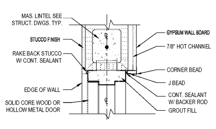
17 JAMB DETAIL SCALE: 1/12"=1'-0"
