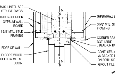
12 HEAD DETAIL SCALE: 1/12"=1'-0"
