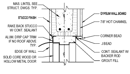
16 HEAD DETAIL SCALE: 1/12"=1'-0"
