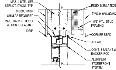
21 HEAD DETAIL SCALE: 1/12"=1'-0"
