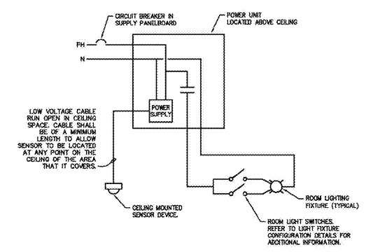
9 E-601 NOT TO SCALE DETAIL - OCCUPANCY SENSOR CONTROL
