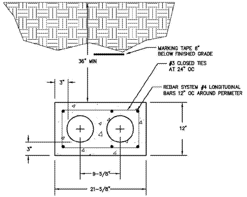
8 E-601 NOT TO SCALE DETAIL - TELECOM SERVICE DUCTBANK
