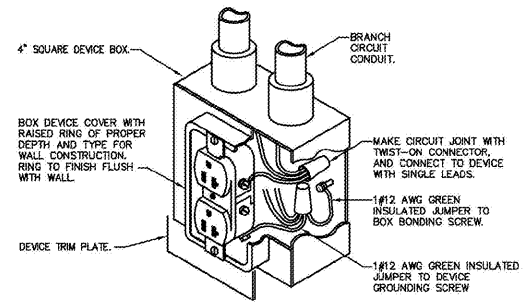
1 E-601 NOT TO SCALE DETAIL - TYPICAL DUPLEX RECEPTACLE INSTALLATION
