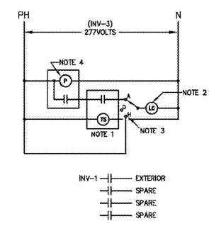
2 E-601 NOT TO SCALE EXTERIOR LIGHTING CONTROL DIAGRAM - ELC
