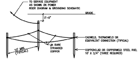
3 E-601 NOT TO SCALE TYPICAL MADE GROUNDING ELECTRODE
