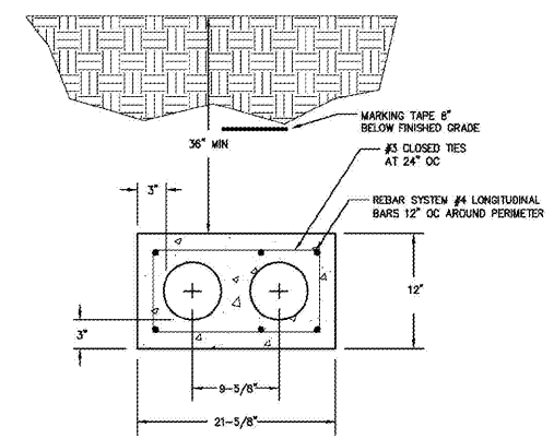
8 E-601 NOT TO SCALE DETAIL - TELECOM SERVICE DUCTBANK
