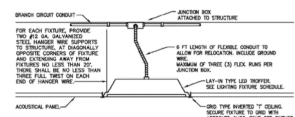
6 E-601 NOT TO SCALE DETAIL - TYPICAL LAY-IN FIXTURE INSTALLATION
