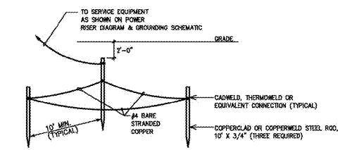
3 E-601 NOT TO SCALE TYPICAL MADE GROUNDING ELECTRODE
