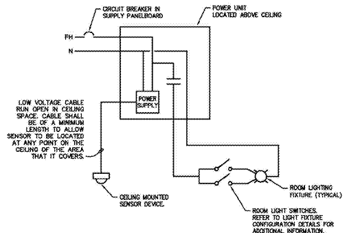
9 E-601 NOT TO SCALE DETAIL - OCCUPANCY SENSOR CONTROL
