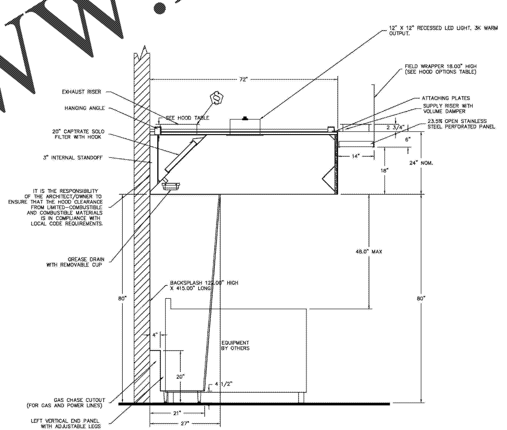
SECTION VIEW - MODEL 7224ND-2-PSP-F HOOD - #2 (#221)
