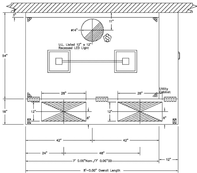
PLAN VIEW - Hood #1 (#112) 7' 0.00" LONG 5424ND-2-PSP-F
