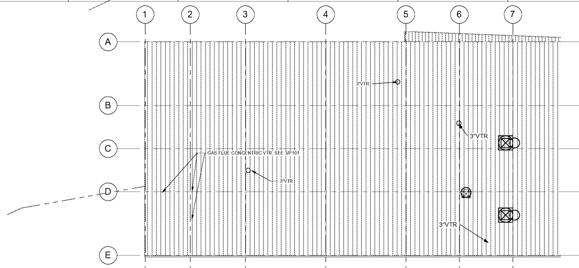
2 PARTIAL ROOF PLAN P-300 3/32" = 1'-0"
