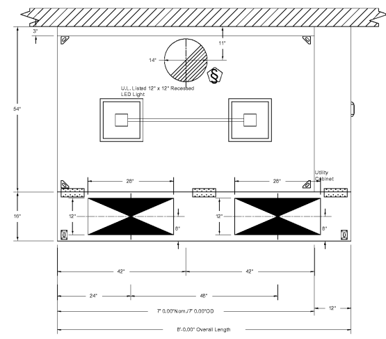
PLAN VIEW - Hood #1 (#112) 7' 0.00" LONG 5424ND-2-PSP-F
