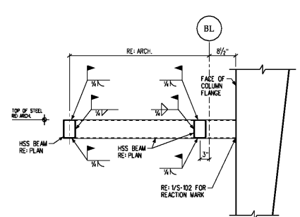
15 Section 3/8" = 1'-0"
