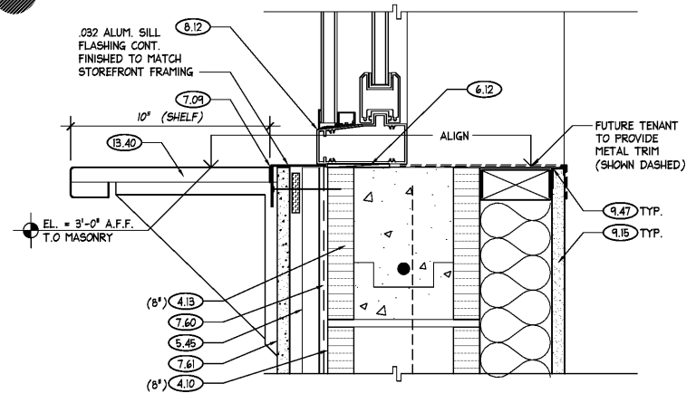
9 DRIVE-THRU SILL DETAIL SCALE: 3" = 1'-0"
