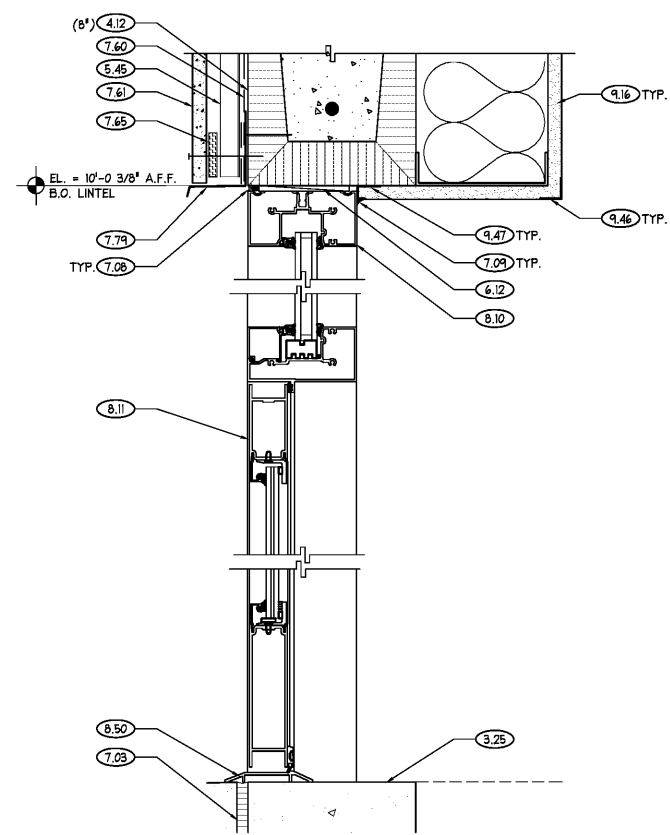
1 STOREFRONT HEAD/ THRESHOLD DETAIL SCALE: 3" = 1'-0"
