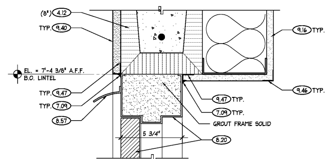
5 DOOR HEAD DETAIL SCALE: 3" = 1'-0"
