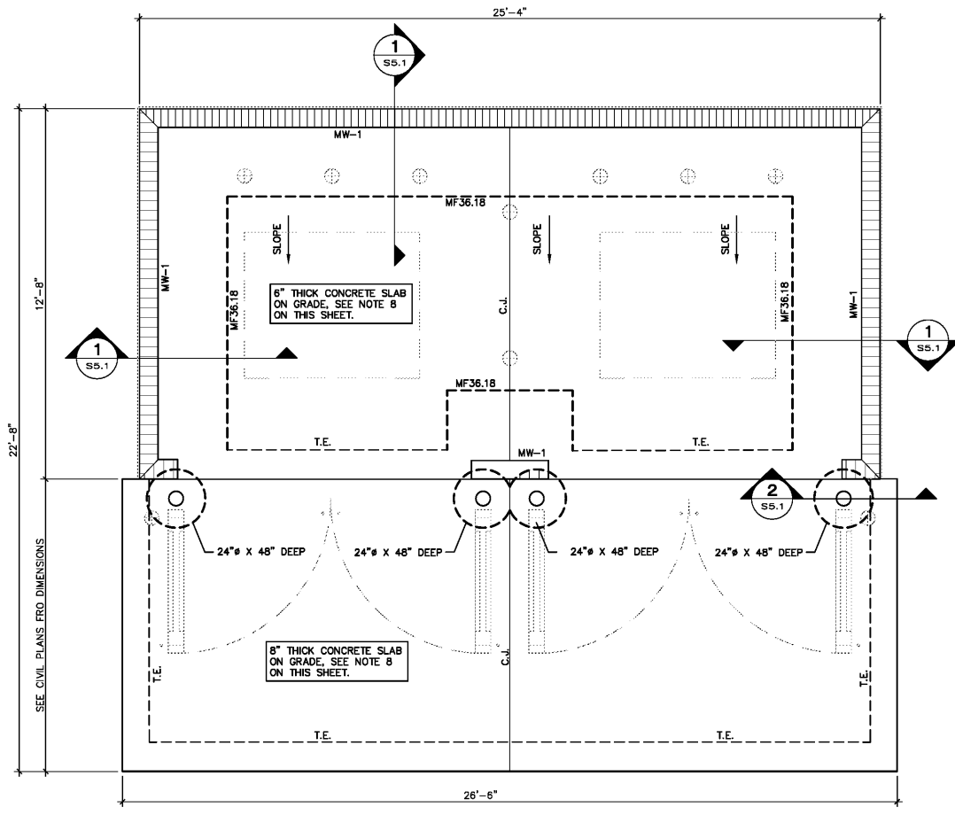
1 DUMPSTER ENCLOSURE - FOUNDATION PLAN 3/8" = 1'-0"
