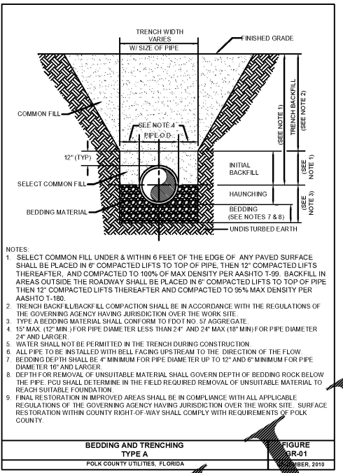
3 TRENCH NTS
