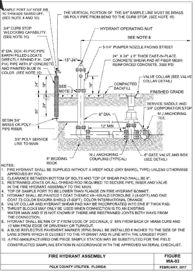
7 FIRE HYDRANT NTS
