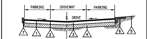
1 TYPICAL PAVEMENT SECTION
