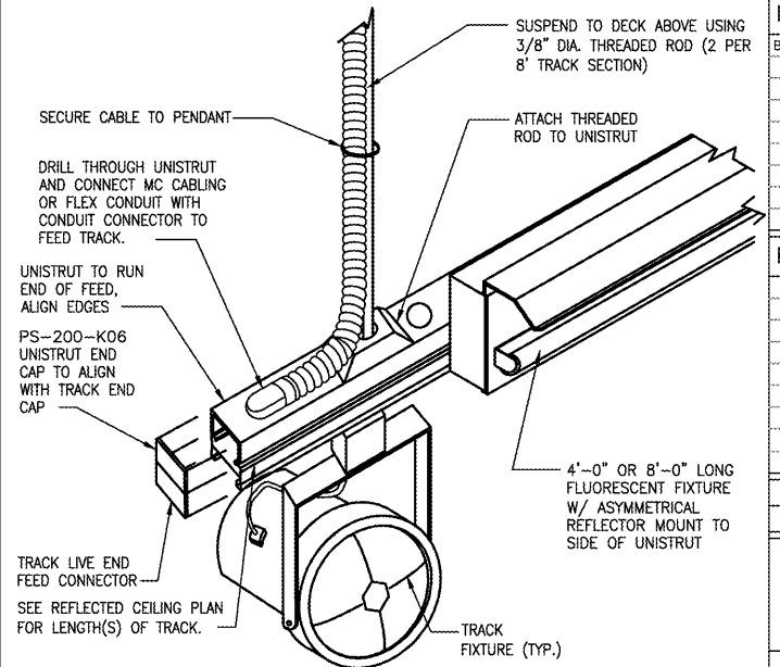
PERIMETER LIGHT AND TRACK LIGHTING DTL.
