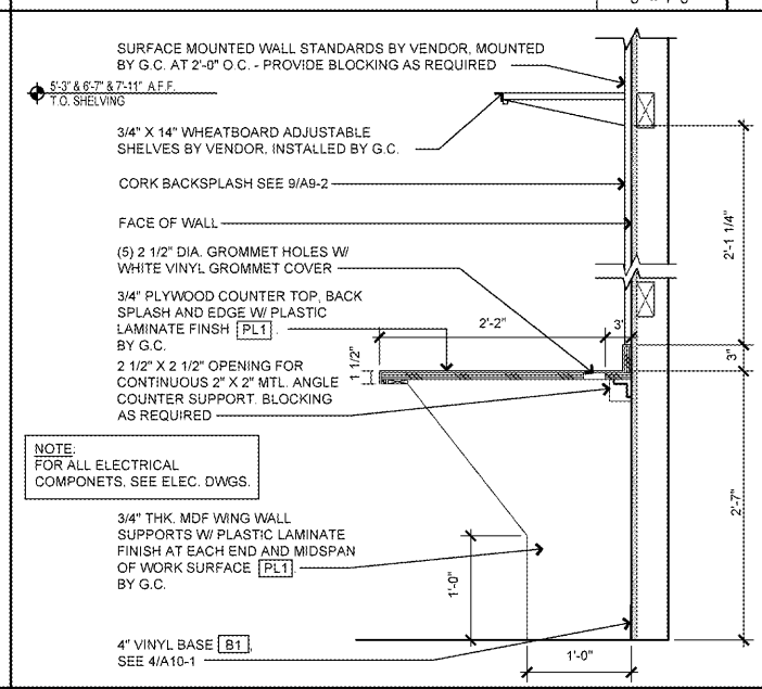
SCALE: 4 MANAGER'S OFFICE COUNTERTOP
