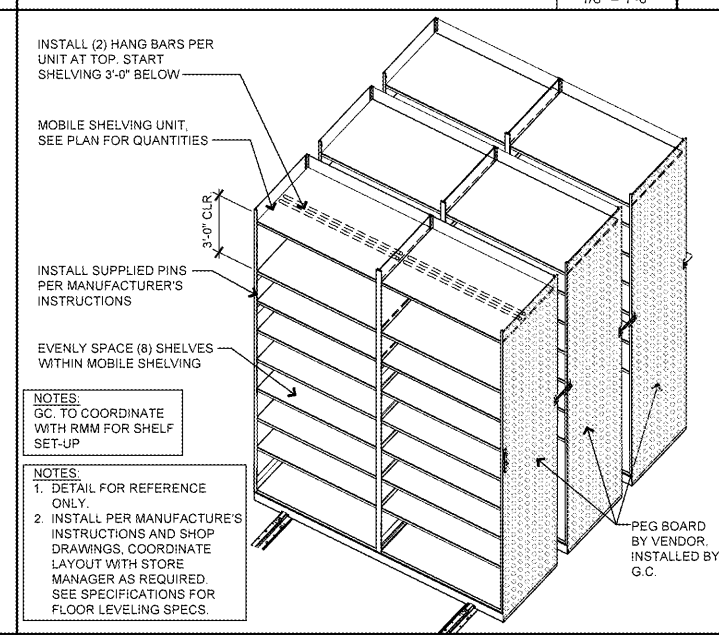
SCALE: 1 MOBILE SHELVING UNIT
