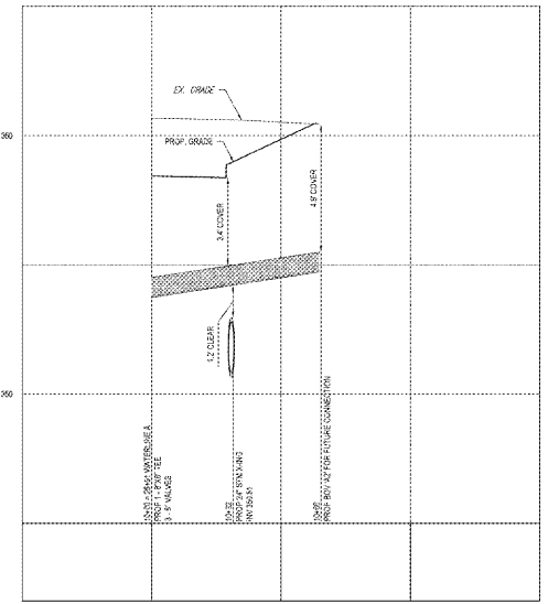
PROPOSED BOV 'A2' PROFILE SCALE: 1"=30' HORIZONTAL 1"=3' VERTICAL
