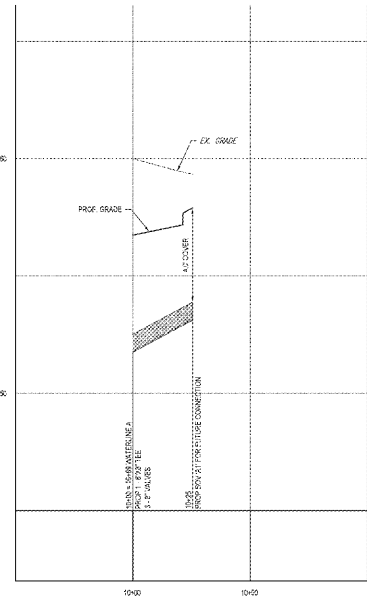
PROPOSED BOV 'A1' PROFILE SCALE: 1"=30' HORIZONTAL 1"=3' VERTICAL
