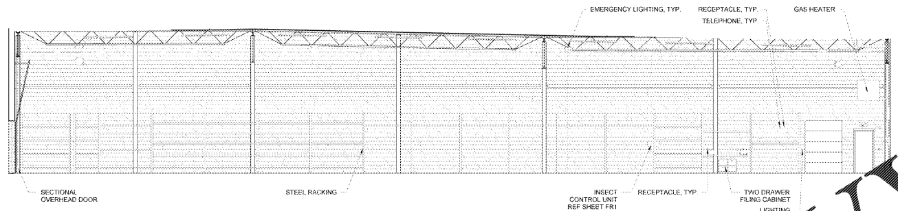
3 ENLARGED RECEIVING ELEVATION 1/4" = 1'-0"
