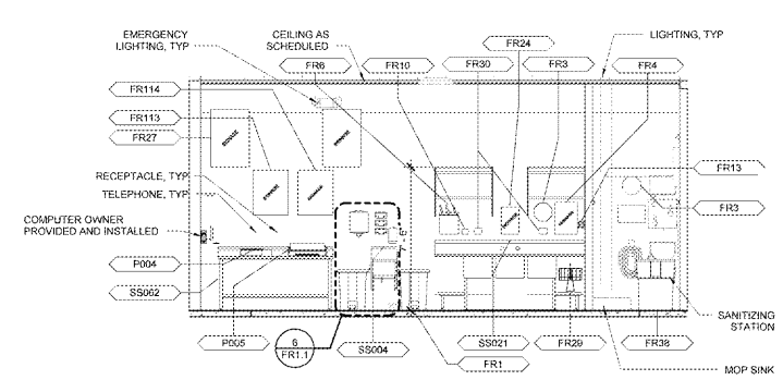
2 ENLARGED PRODUCE PREP ELEVATION 1/4" = 1'-0"
