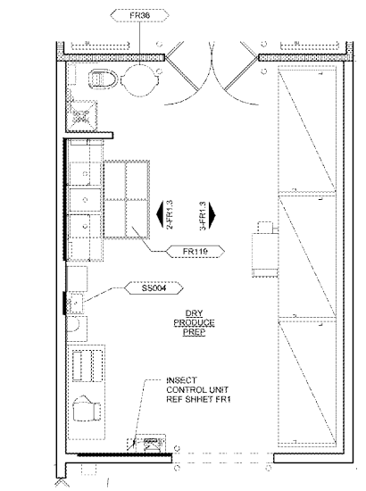
1 ENLARGED PRODUCE PREP PLAN 1/4" = 1'-0"
