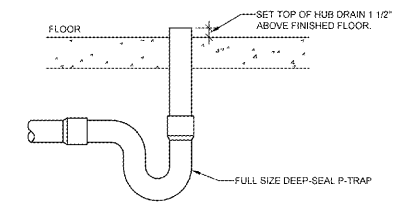
5 HUB DRAIN NTS
