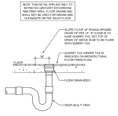
4 OPEN FLOOR AREA DRAIN NTS
