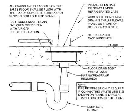
3 REFRIGERATED CASE DRAIN NTS
