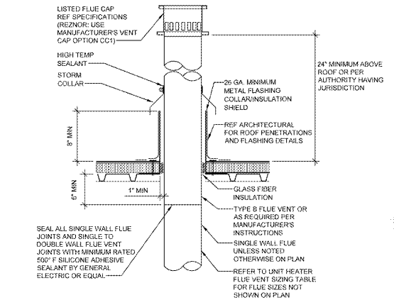
7 GAS RADIANT HEATER CONNECTION NTS
