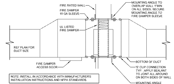
9 FIRE DAMPER NTS
