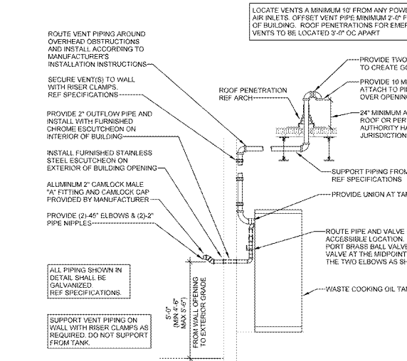
14 WASTE COOKING OIL TANK PIPING NTS
