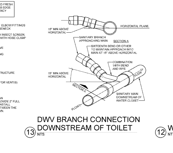
13 DWV BRANCH CONNECTION DOWNSTREAM OF TOILET NTS
