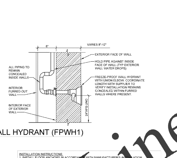
12 WALL HYDRANT (FPWH1) NTS
