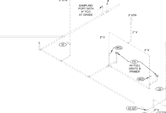
4 REAR OFFICE/RESTROOM DWV RISER NTS
