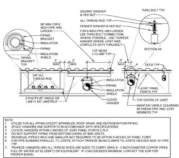
15 PIPE SUPPORT NTS
