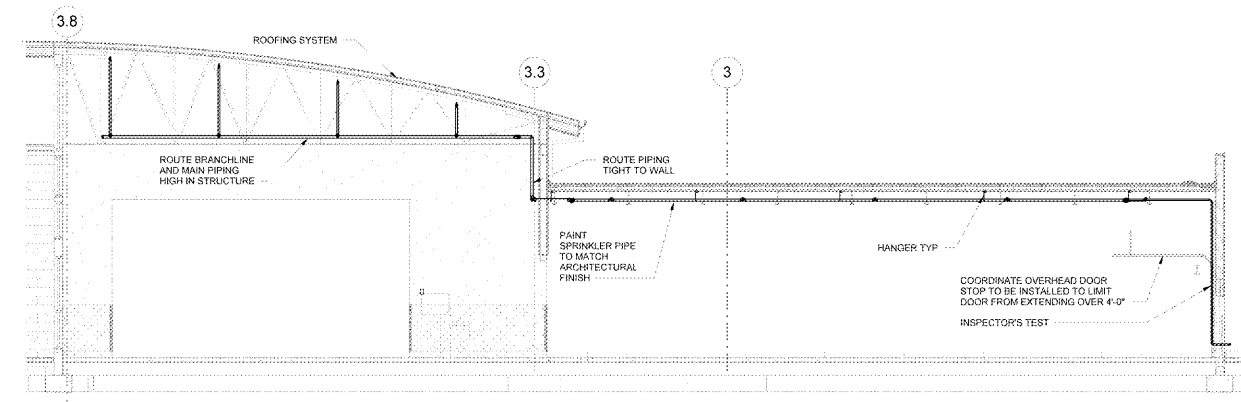
3.8 GR VESTIBULE SECTION NTS
