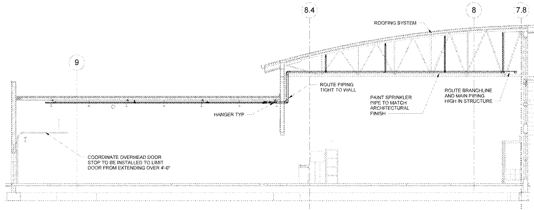
3 GM VESTIBULE SECTION NTS
